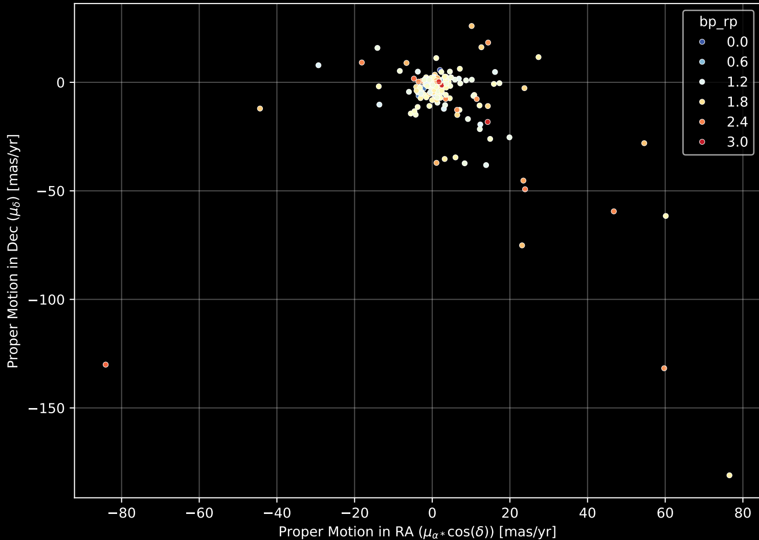
APOGEE DR17 Field: [Berkeley_20_btx] Proper Motion Diagram (n= 309)
