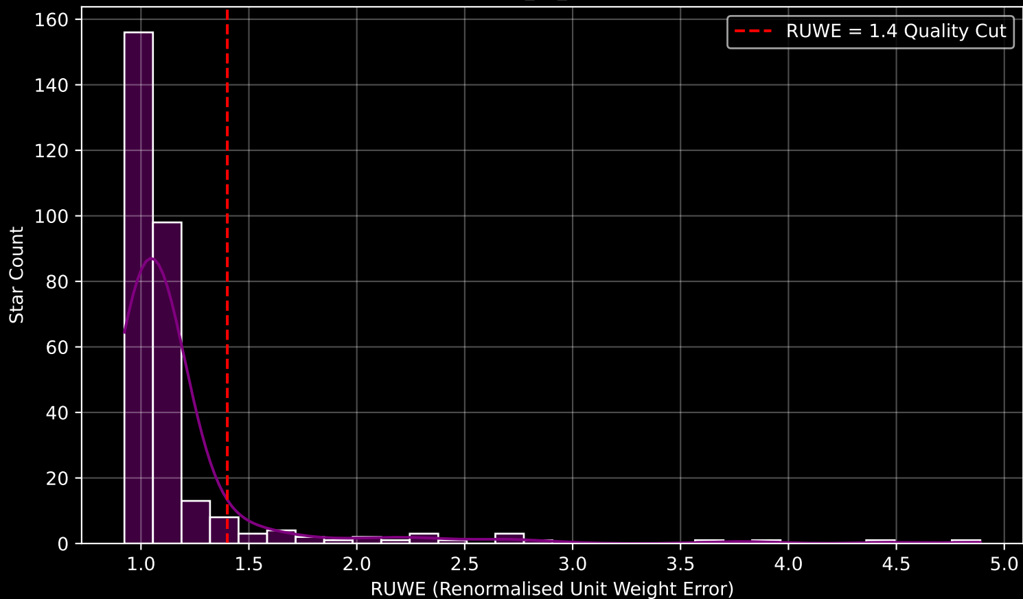
GAPOGEE DR17 Field [Berkeley_20_btx] RUWE Distribution (n= 300)
