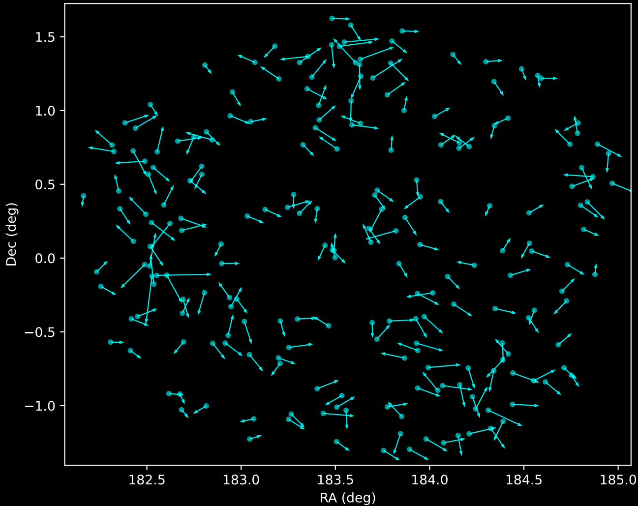
APOGEE DR17 Noise Stream Proper Motion Vectors (n=213)
