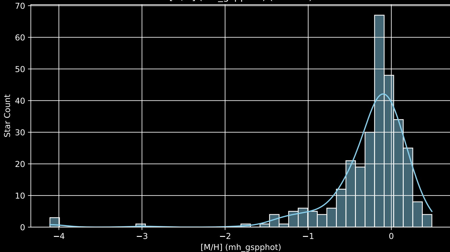
APOGEE DR17 Field: [Berkeley_20_btx [M/H] (mh_gspphot) (n= 305)
