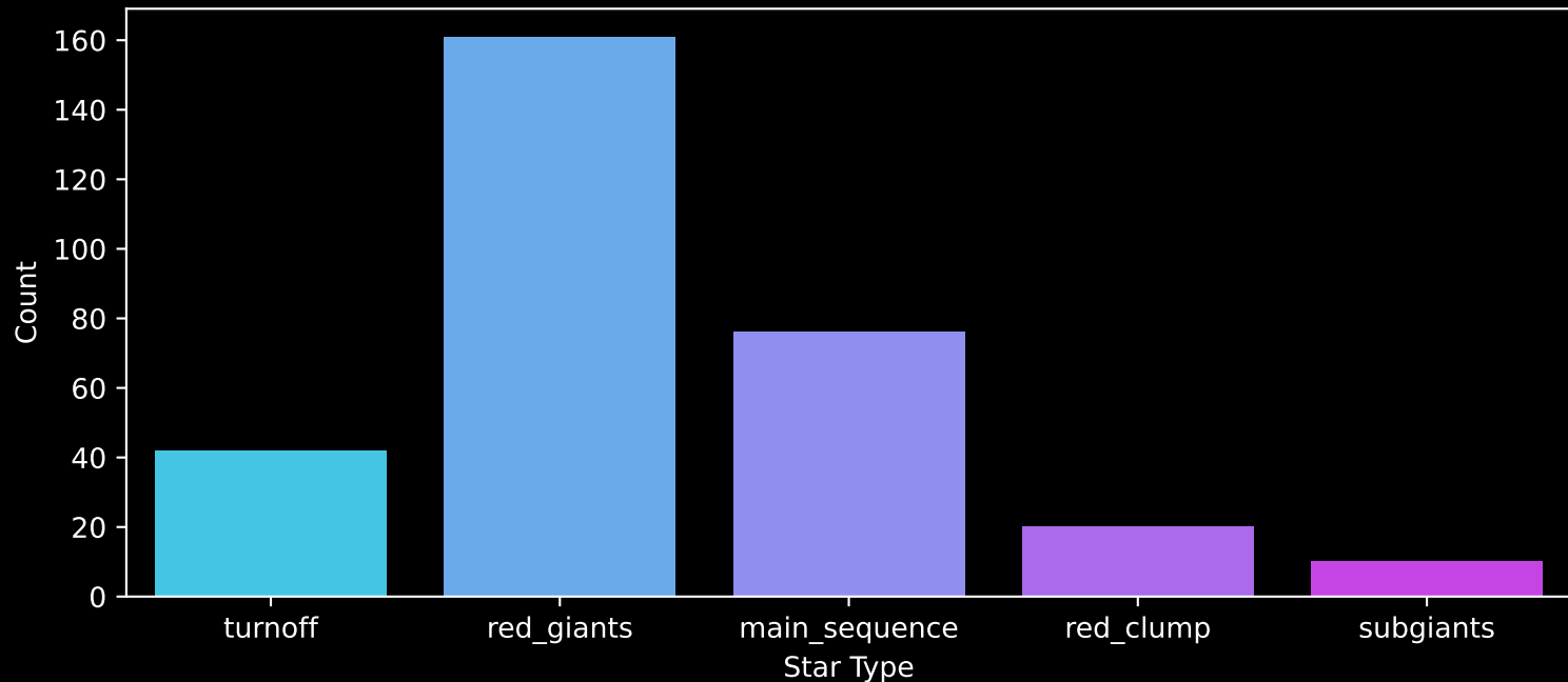
APOGEE DR17 Field: [Berkeley_20_btx] Count plot of Star Type
