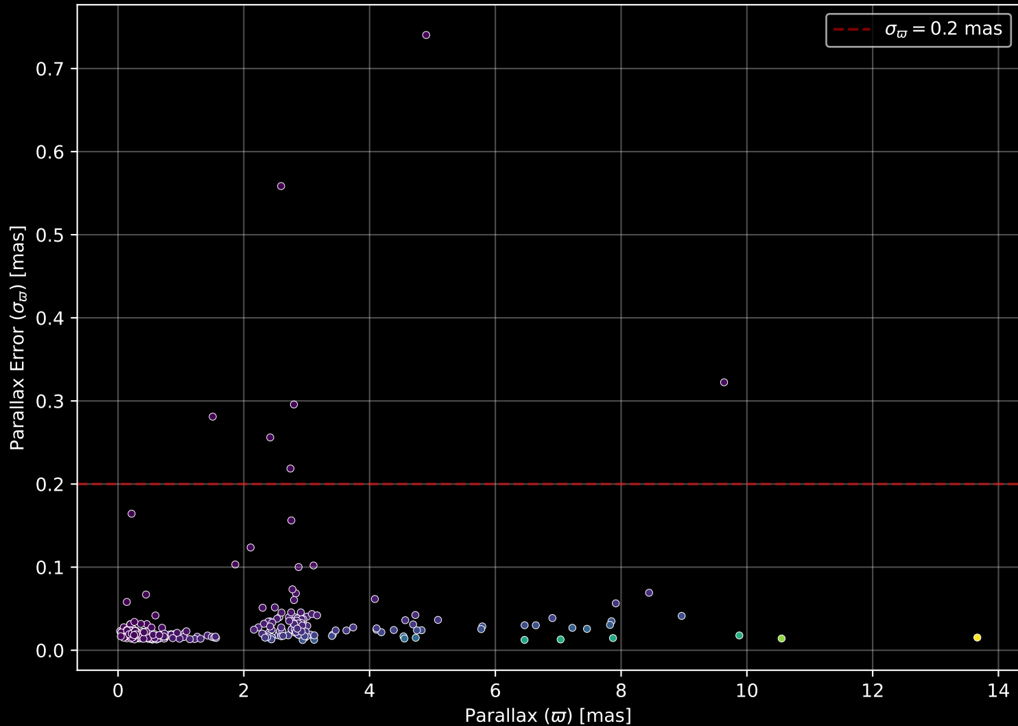
APOGEE DR17 Field: [Berkeley_20_btx] Parallax Quality (n= 309)
